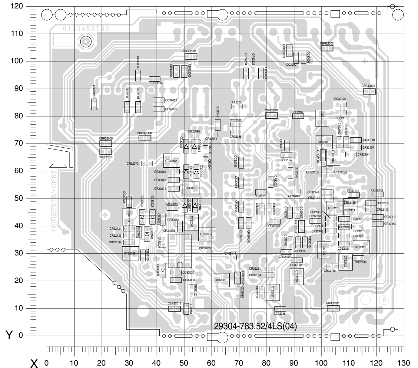
Coordinates of the components on the Solder Side (Bottom Side)
